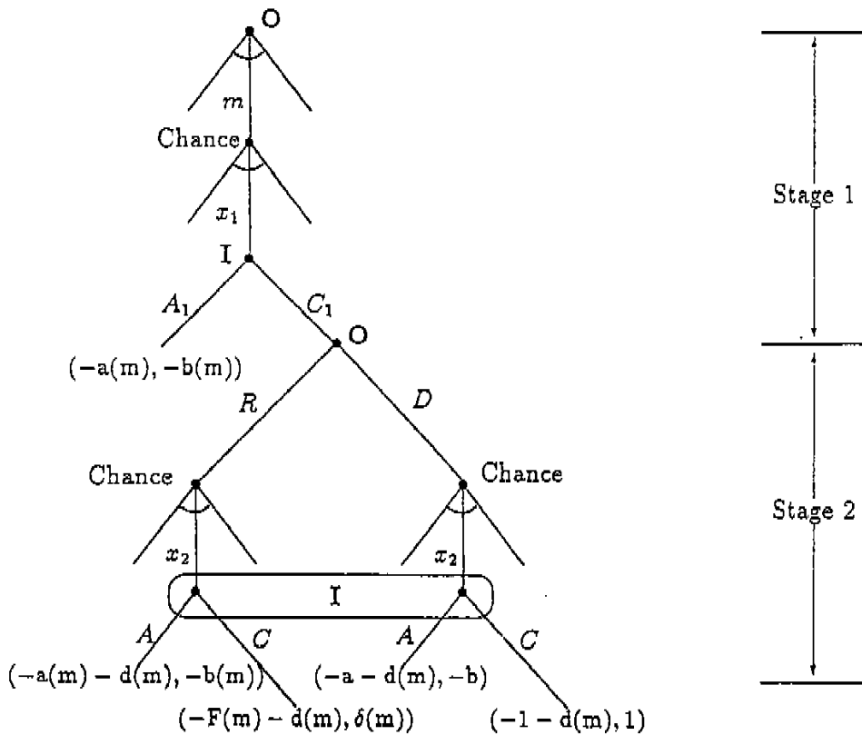
Figure 5: The extensive form game.
