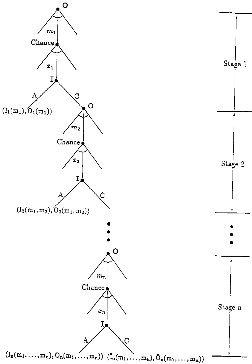
Figure 1: The game in extensive form.
