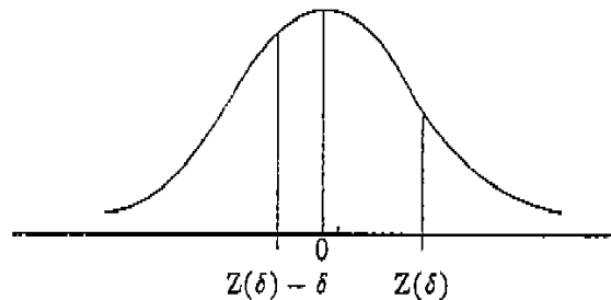
Figure 6: The Standard Normal Distribution.
