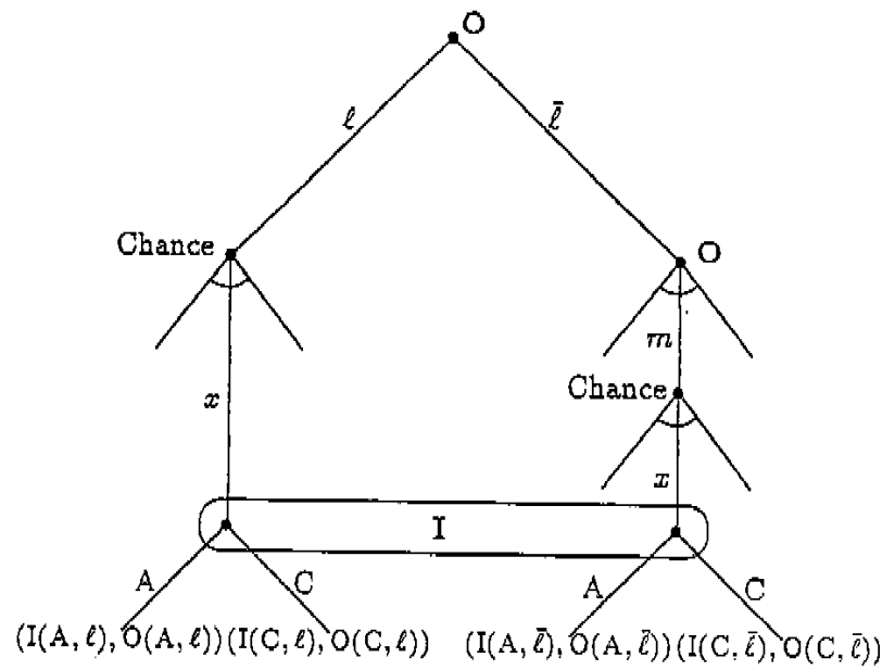
Figure 2: The restricted game \Gamma_0 in extensive form.
