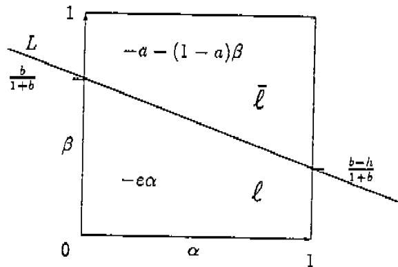
Figure 3: Payoff for I in \Gamma_0 , when I uses (\alpha, \beta) test and O plays a best reply.
